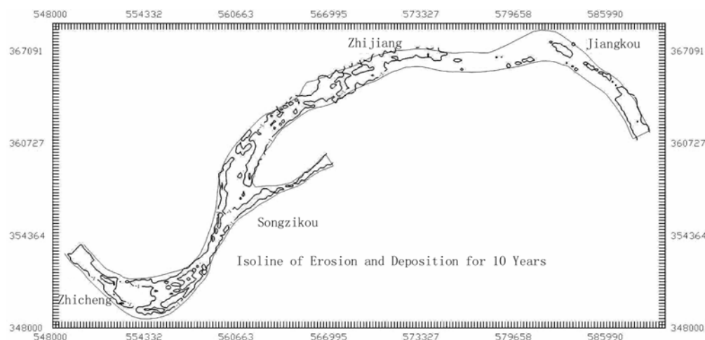
Fig. 6 Isolines of 1 m and 3 m of erosion in Zhicheng-Dabujie reach after 10 years
